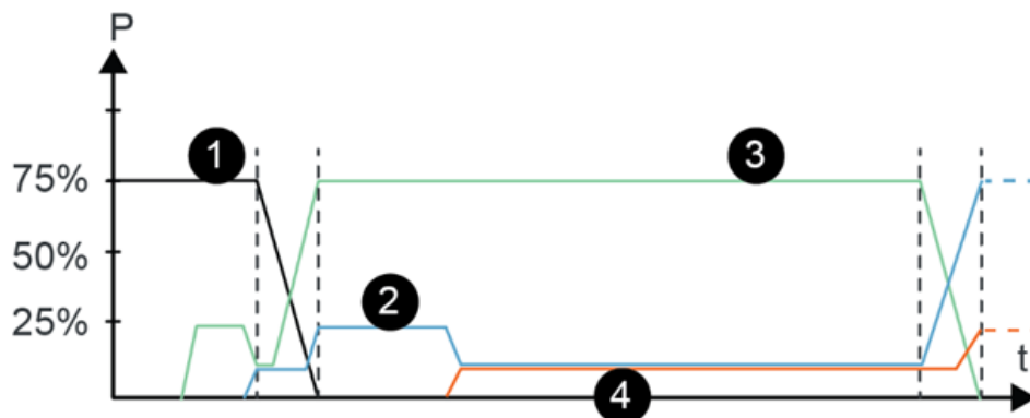
Figure 9. Power at the charging station outputs
