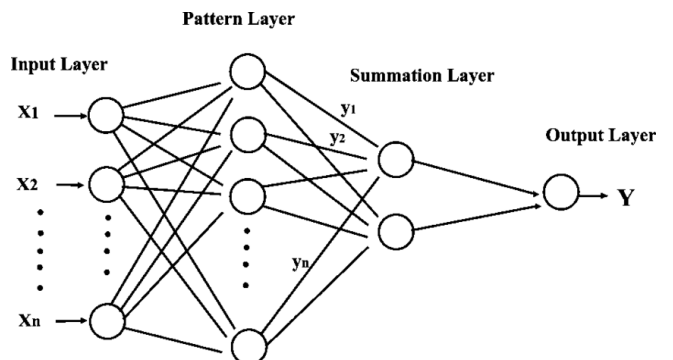
Figure 5. Generalized regression artificial neural network structure (Usluoglu et al. 2008)
