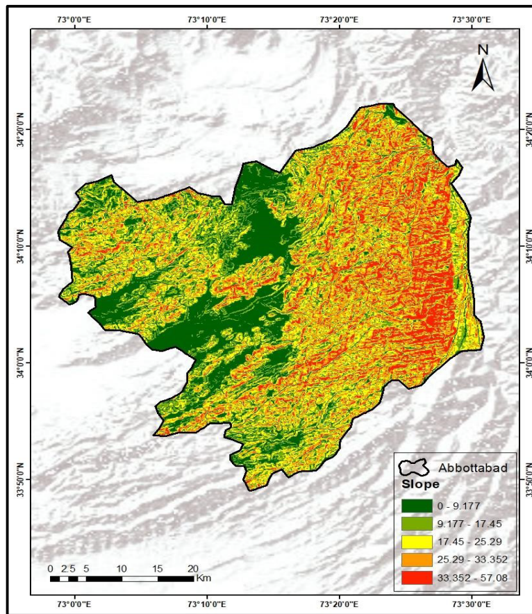
Figure 2. Slope of Abbottabad District.
